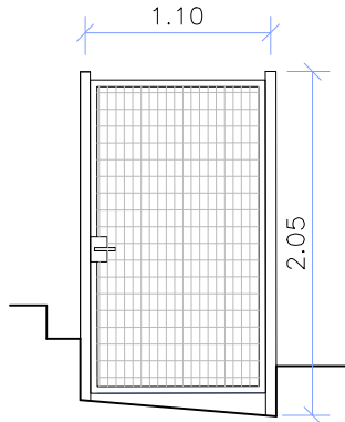
S1-P1 Porta vianants tanca perimetral
